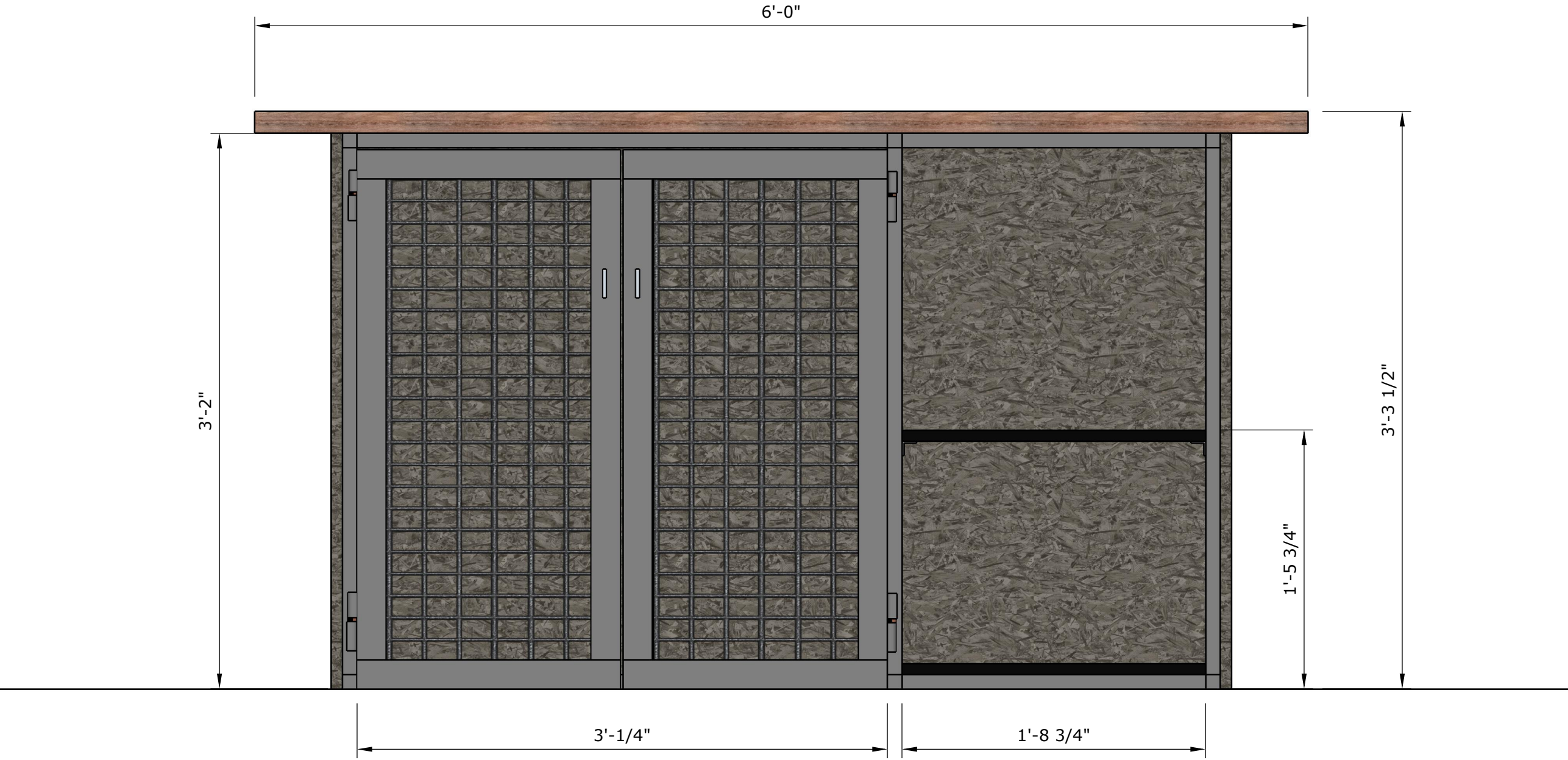
FRONT ELEVATION
