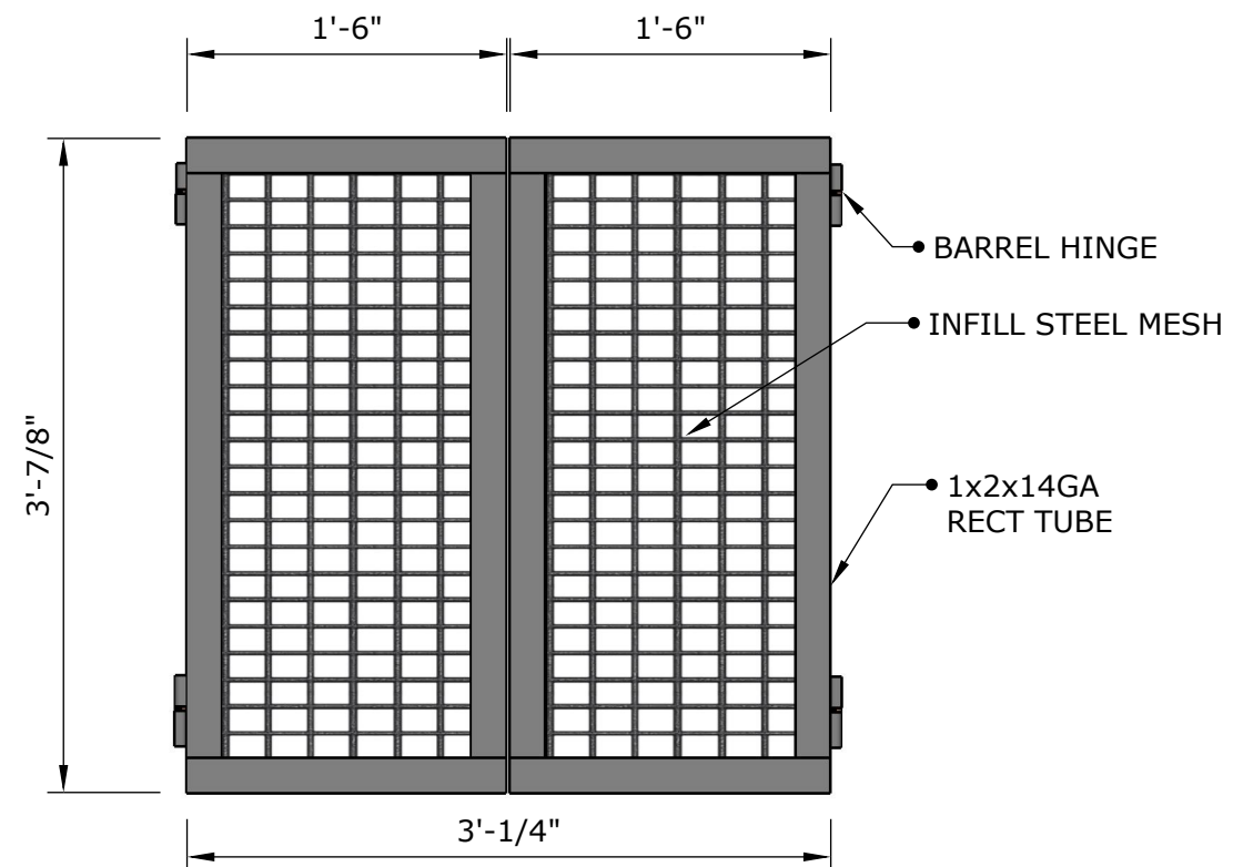
CABINET DOOR ELEVATION
