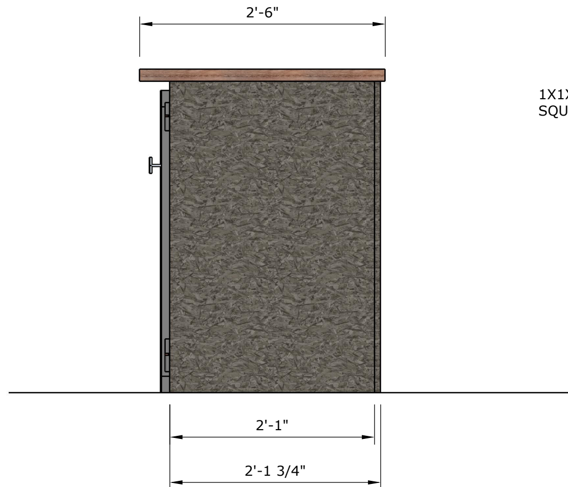
SIDE ELEVATION
