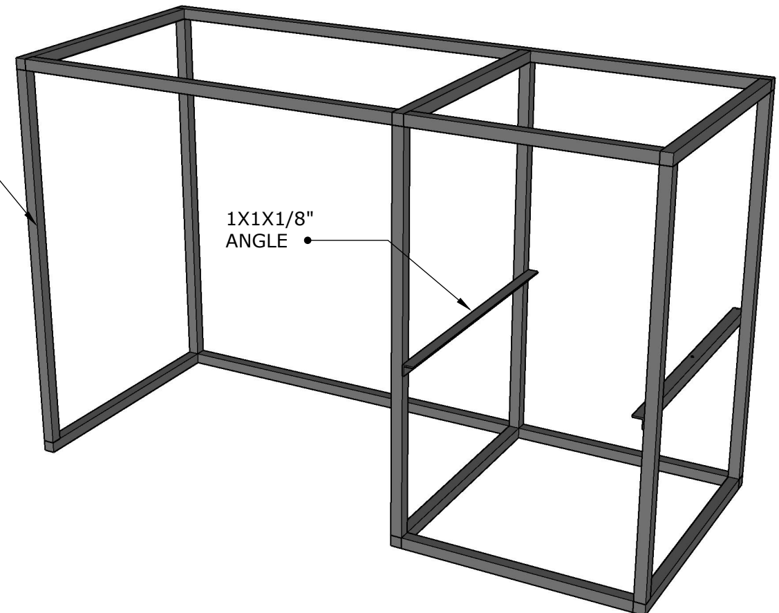
FRAME ISOMETRIC
